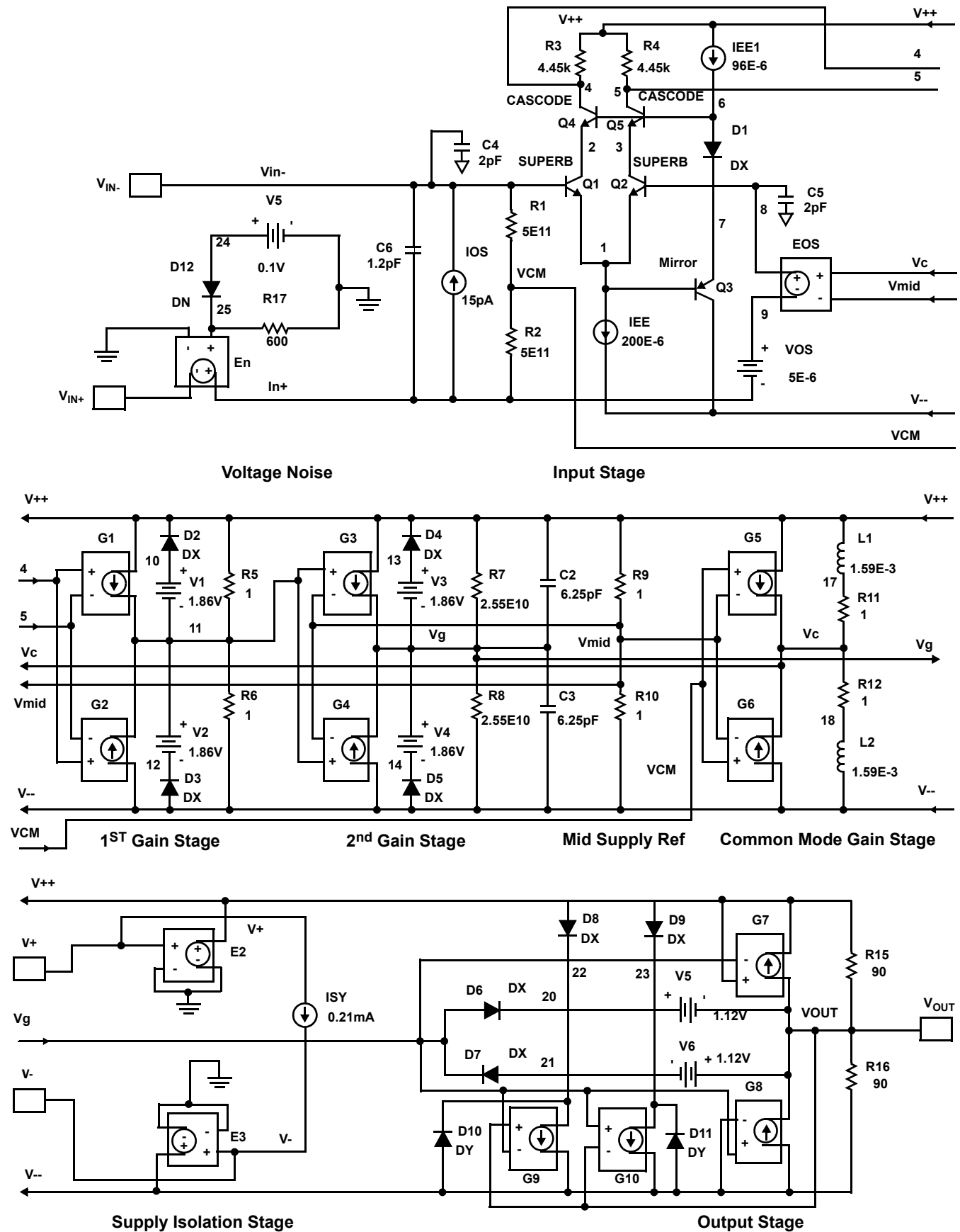
FIGURE 56. SPICE SCHEMATIC
