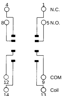
Schematic
