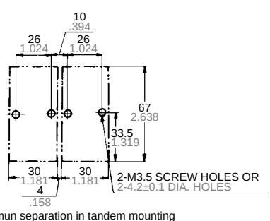
Chassis cutout
