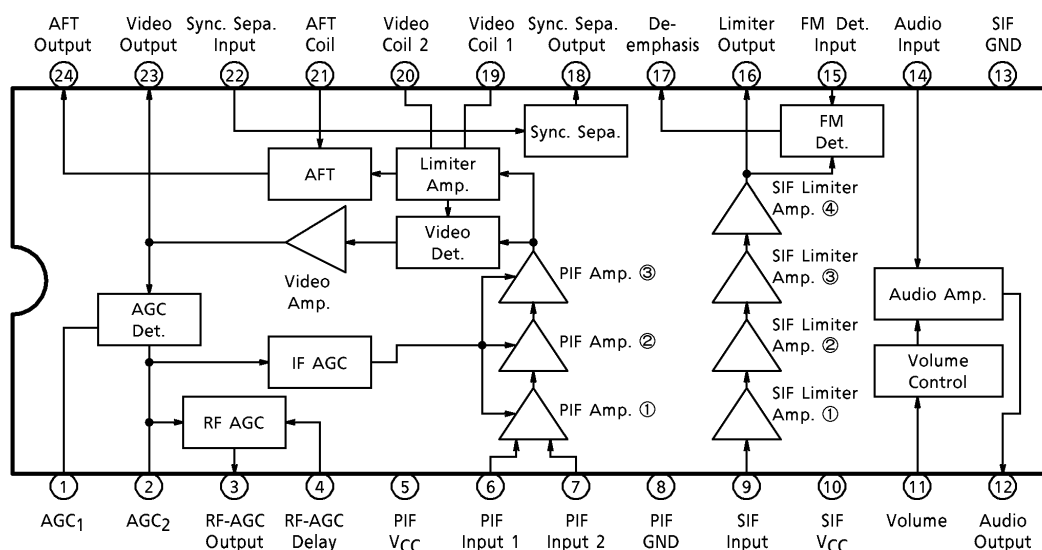
BLOCK DIAGRAM (TA8836F, TA1207F)
