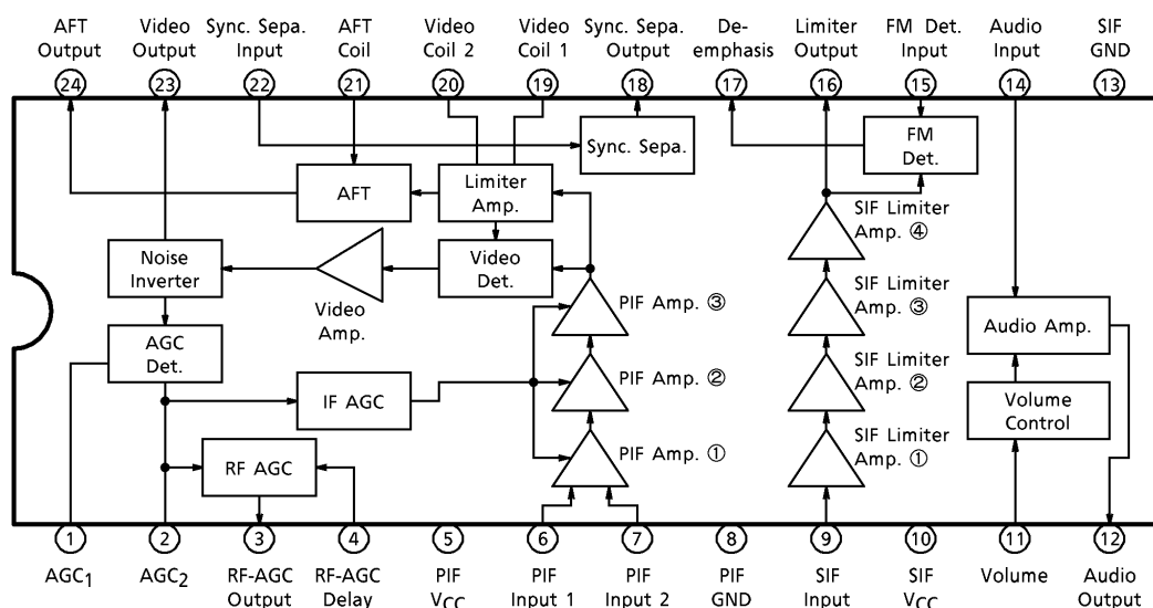
BLOCK DIAGRAM (TA8805F)
