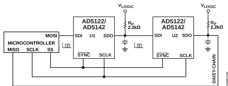
Figure 39. Daisy-Chain Configuration
