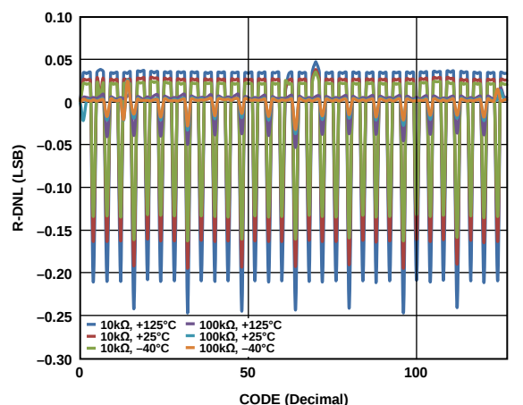
Figure 12. R-DNL vs. Code (AD5122)
