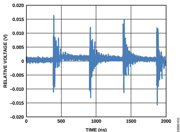
Figure 31. Digital Feedthrough
