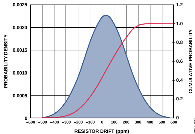
Figure 29. Resistor Lifetime Drift
