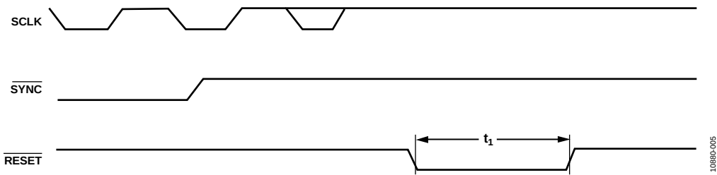
Figure 5. Control Pins Timing Diagram
