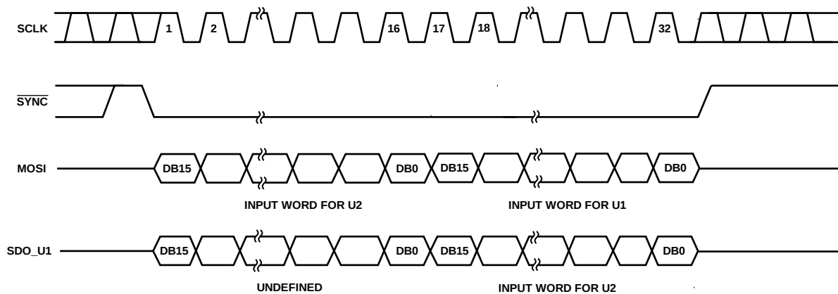
Figure 40. Daisy-Chain Diagram
