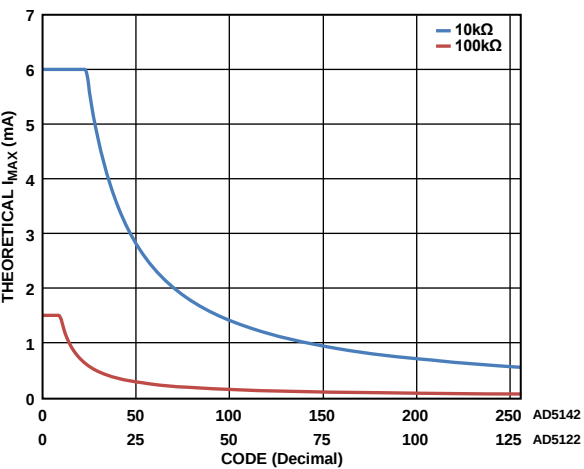
Figure 33. Theoretical Maximum Current vs. Code
