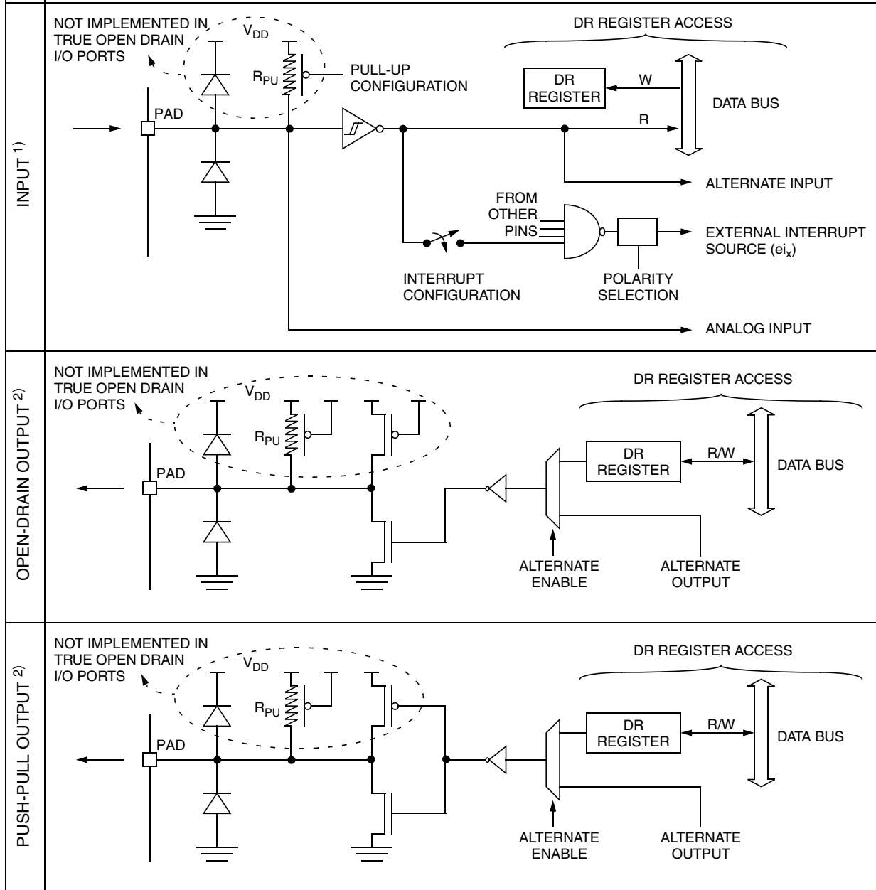
Hardware Configuration
