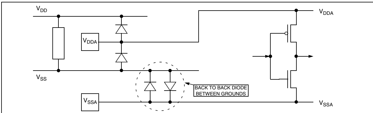
Figure 77. Multisupply Configuration
