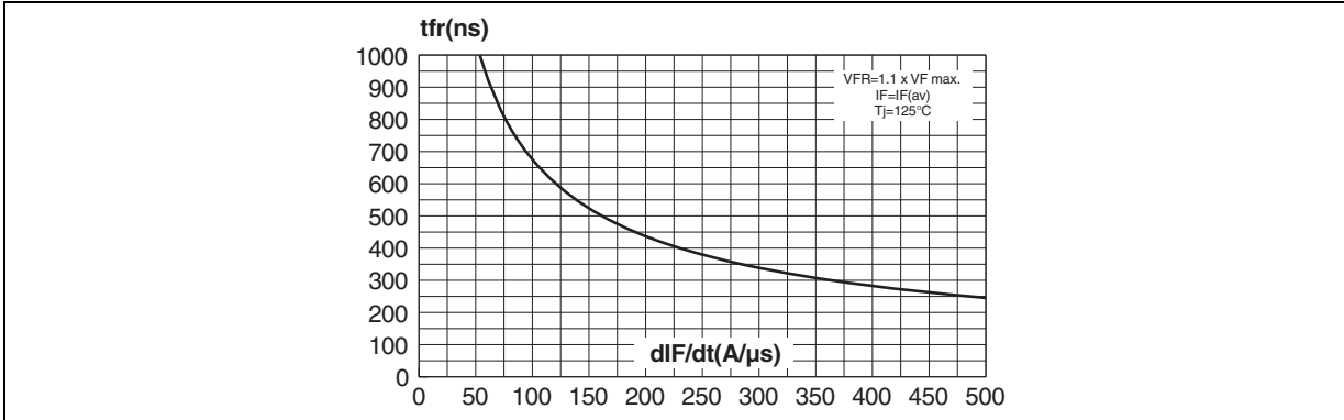
Figure 9. Forward recovery time versus dl_F/dt (90% confidence, per diode)
