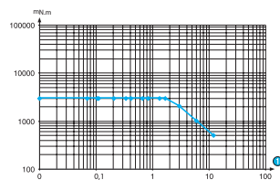
Torque / speed curves 80 523 0
