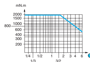
Graph of torque versus speed 82 305 0
