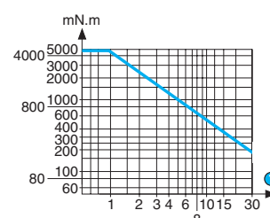
Torque/speed curves 80 527 0
