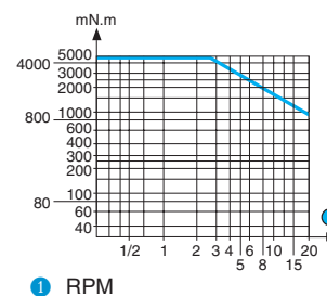
Torque/speed curves 80 547 0
