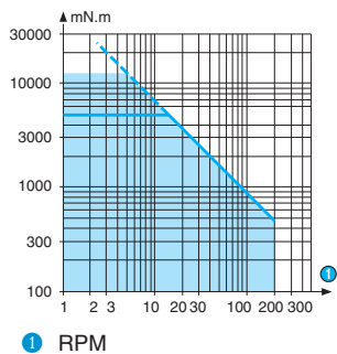
Nominal speed and torque curves 80 807 0
