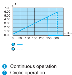
Current/torque
