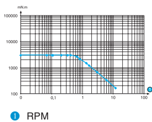
Torque / speed curves 80 513 0
