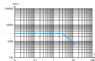
Torque / speed curves 80 533 0
