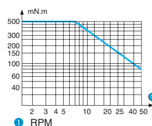
Graph of torque versus speed 82 514 5
