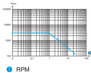
Torque / speed curves 80 513 5
