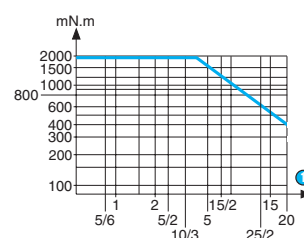
Torque/speed curves 82 529 4
