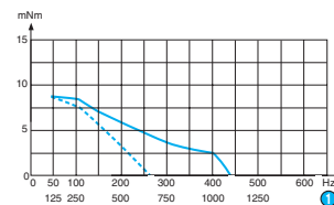
Nominal value dynamic curves 4 phases - 115 \Omega
