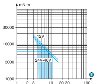
Nominal speed and torque curves 82 812 5
