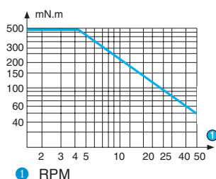
Graph of torque versus speed 82 514 0
