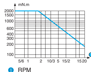
Graph of torque versus speed 82 519 5
