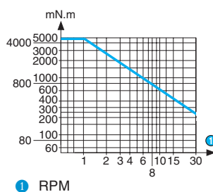
Torque/speed curves 80 527 4
