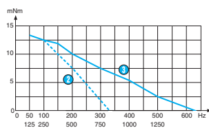
Nominal value dynamic curves 2 phases - 12.9 \Omega
