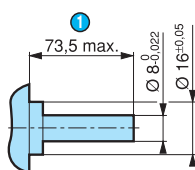
Gearbox shaft 79 290 064
