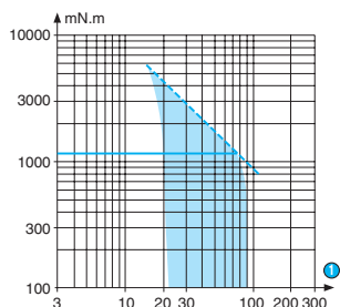
Nominal speed and torque curves 82 802 0
