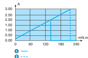
Current/torque
