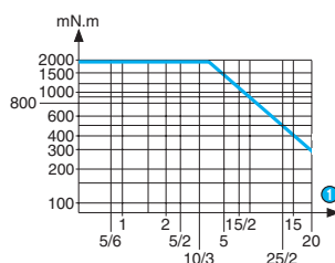
Torque/speed curves 82 529 0
