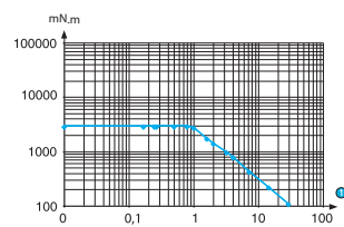
Graph of torque versus speed 82 333 5
