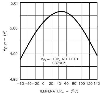
FIGURE 3. TEMPERATURE COEFFICIENT
