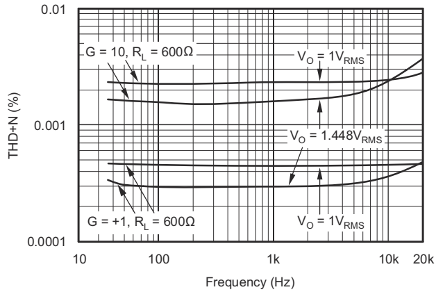
Figure 6-13. Total Harmonic Distortion + Noise vs Frequency
