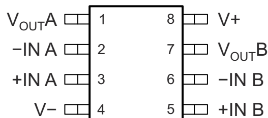
Figure 5-2. D Package 8-Pin SOIC Top View
