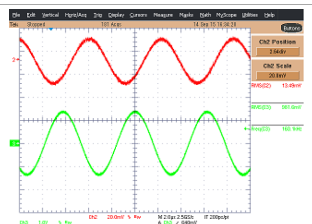
Figure 8-12. Gain Is -3 dB Above the Flat Gain at 160 kHz
