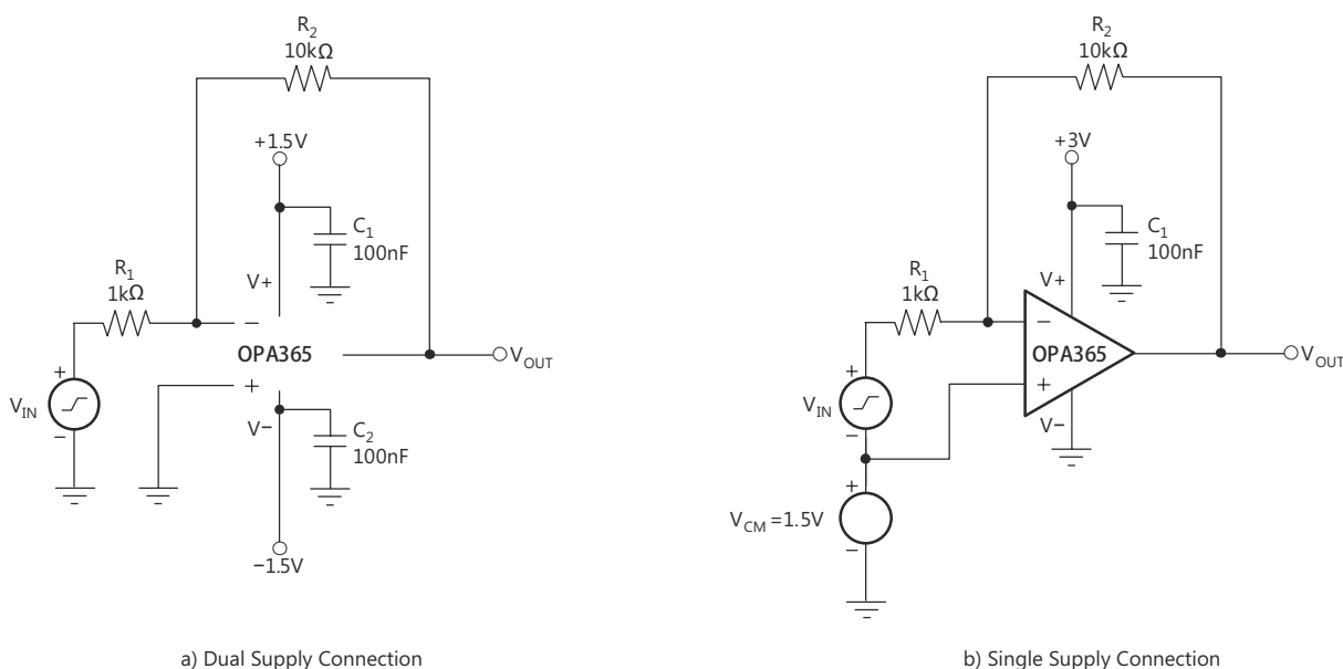
Figure 7-1. Basic Circuit Connections
