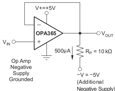
Figure 8-2. Swing-to-Ground
