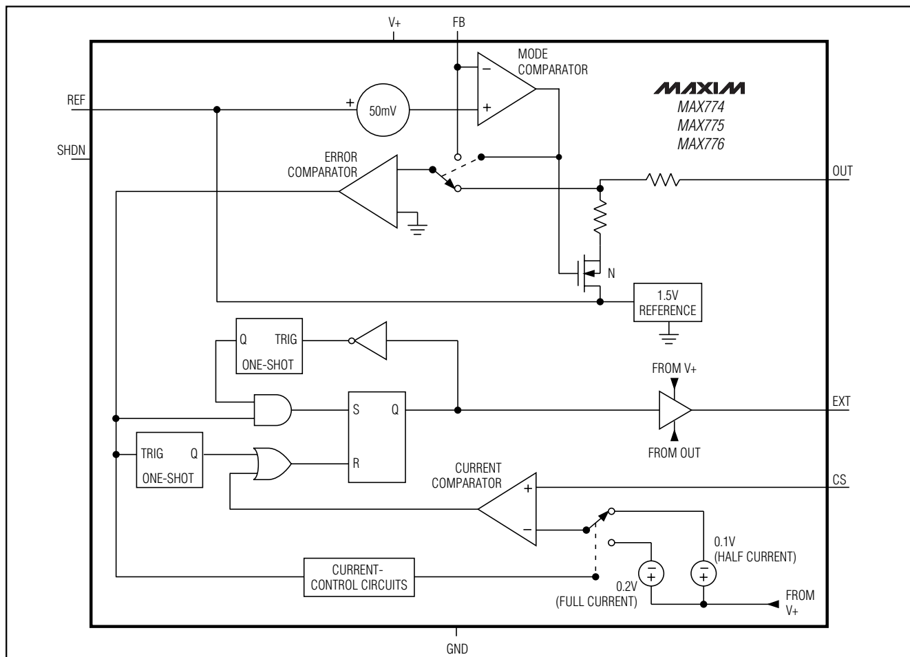
Figure 1. Functional Diagram
