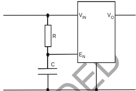
Fig. 1 Circuit Connection
