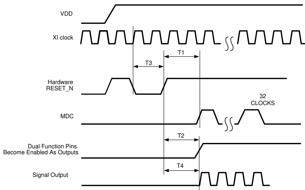
Figure 6-2. Reset Timing
