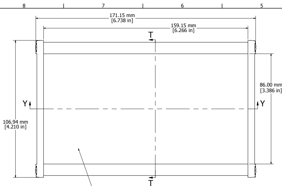
ASSEMBLY - VIEW FROM TOP
