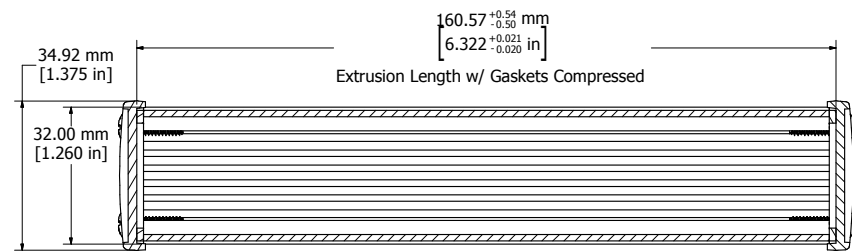
SECTION Y-Y
