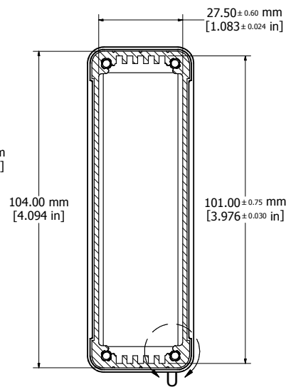
SECTION T-T
