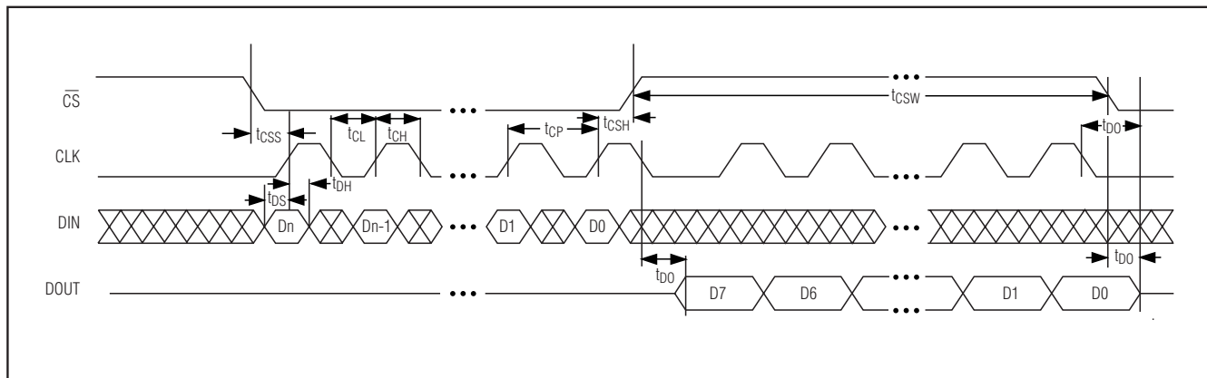
Figure 5. Timing Diagram
