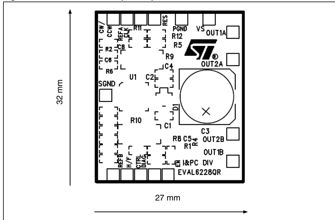
Figure 4. EVAL6228QR component placement
