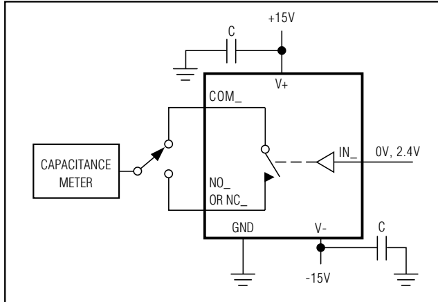
Figure 3. Channel-Off Capacitance
