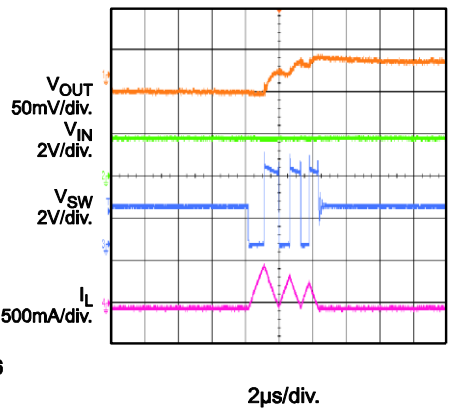
Output Ripple I_{OUT}=0A
