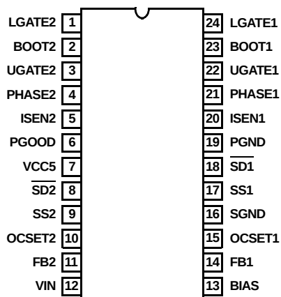
ISL6445 (24 LD QSOP) TOP VIEW
