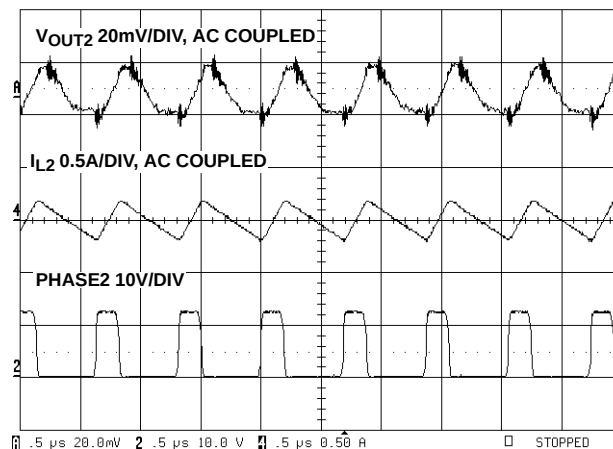
FIGURE 6. PWM2 WAVEFORMS
