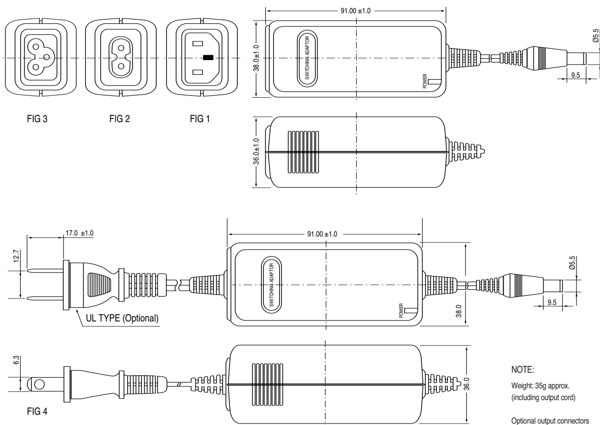
MECHANICAL DIMENSIONS mm
