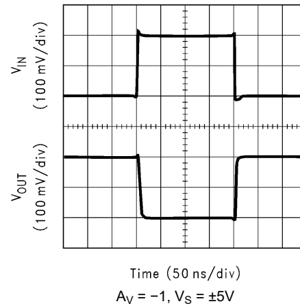
Figure 5-73. Small-Signal Pulse Response
