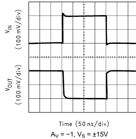
Figure 5-71. Small-Signal Pulse Response
