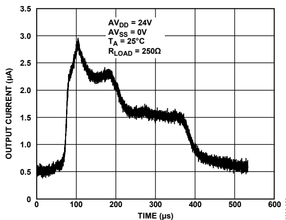
Figure 60. Output Current vs. Time on Power-Up
