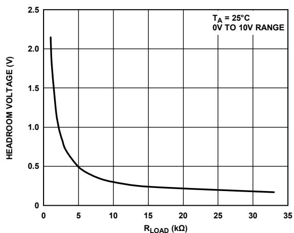
Figure 34. V_{OUT} Headroom
