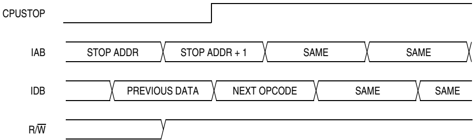
Figure 14-17. Stop Mode Entry Timing
