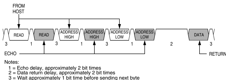
Figure 19-14. Read Transaction
