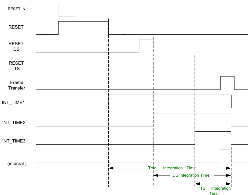
Figure 16. INT_TIME Timing
