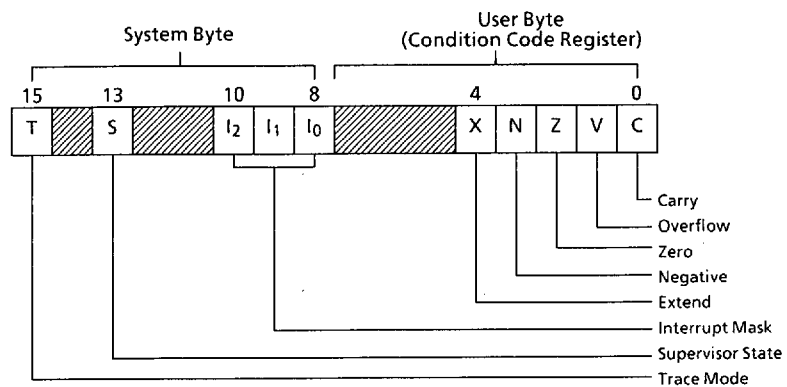
Figure 1.3 Status Register
