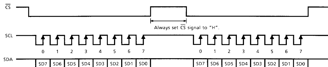
Figure 4 Serial control timing
