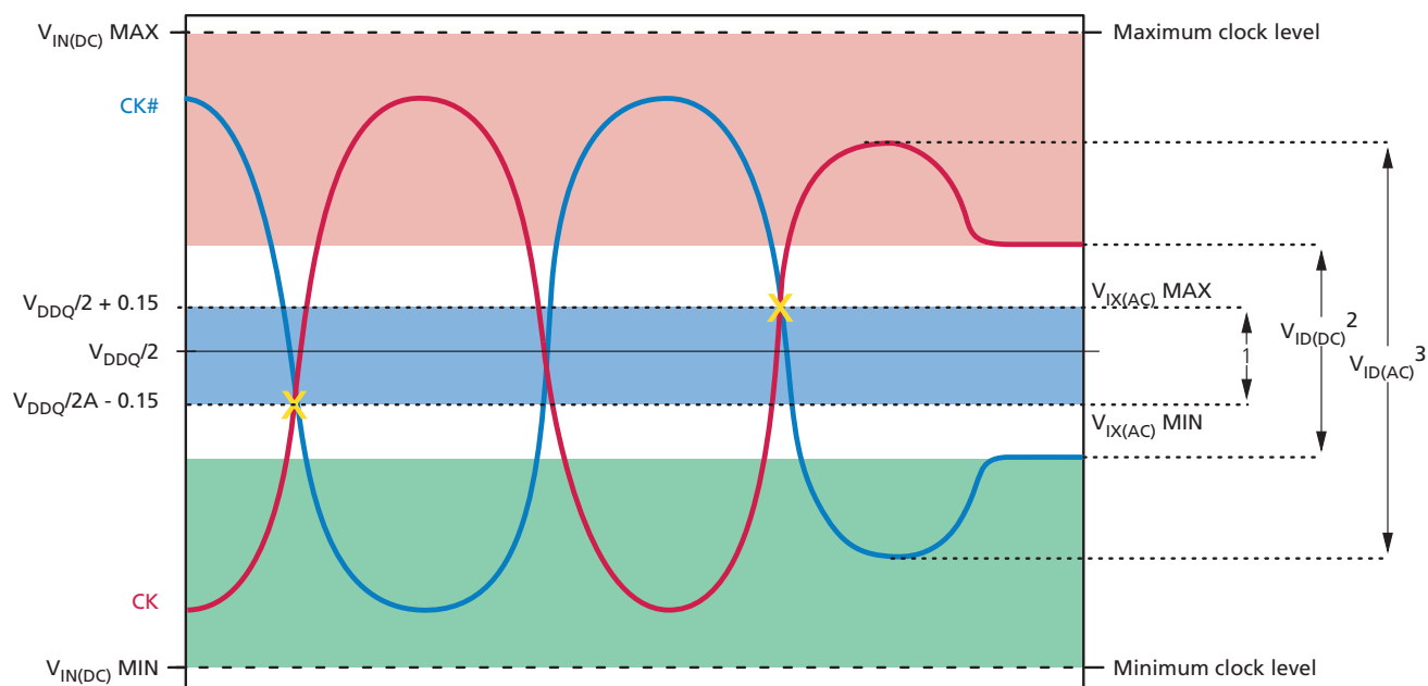
Figure 8: Clock Input
