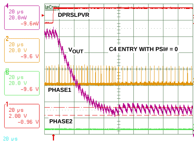
FIGURE 23. C4 ENTRY WITH VID CHANGE OF 011X011 FROM 0.8625V TO 0.7625V, I_{LOAD} = 3A , 1-CCM TO 1-DCM
