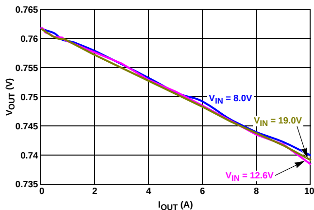
FIGURE 7. DEEPER SLEEP MODE LOAD LINE, 1 PHASE, DCM MODE, VID = 0.7625V
