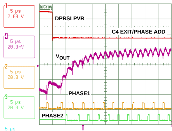
FIGURE 21. VID3 CHANGE OF 010X000 FROM 1.1V TO 1.1V AT DPRSLPVR = 0, DPRSTP# = 1, PSI# = 1
