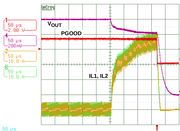
FIGURE 24. OVERCURRENT PROTECTION
