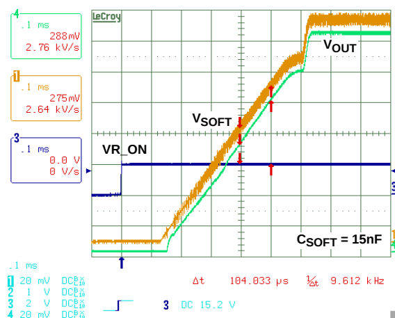
FIGURE 9. SOFT-START WAVEFORM SHOWING SLEW RATE OF 2.5mV/μs AT VID = 1.4375V, I LOAD = 10A
