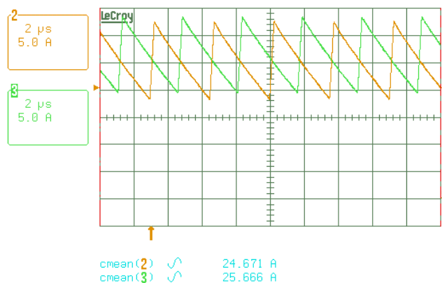
FIGURE 13. 2 PHASE CURRENT BALANCE, FULL LOAD = 50A
