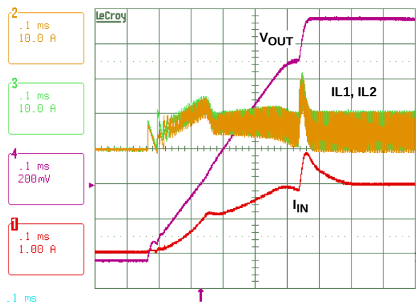
FIGURE 11. INRUSH CURRENT AT START-UP, V IN = 8V, VID = 1.4375V, I LOAD = 10A
