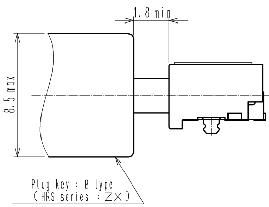
Section of mated condition
