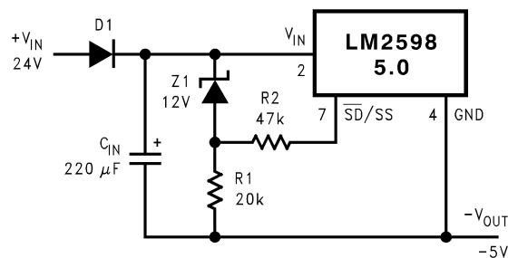
Figure 48. Undervoltage Lockout With Hysteresis for an Inverting Regulator
