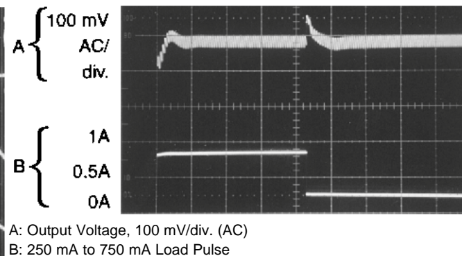
Figure 22. Horizontal Time Base: 100 \mu\text{s}/\text{div} .
