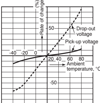
5.-(3) Change of pick-up and drop-out voltage (2 Form A) Tested sample: DSP2a-DC12V, 5 pcs.
