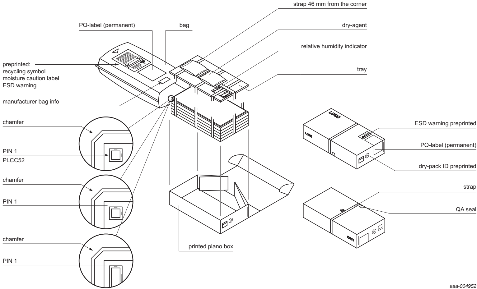
Fig 32. Packing information 5 tray
