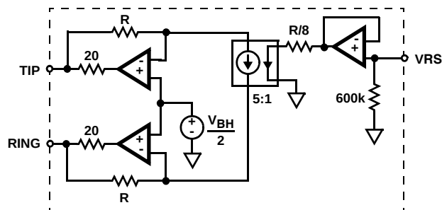
FIGURE 10. LINEAR RINGLING MODEL
