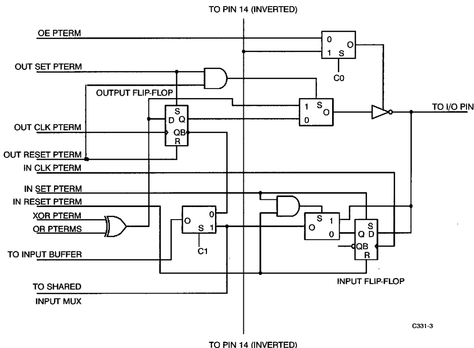
Figure 1. I/O Macrocell
