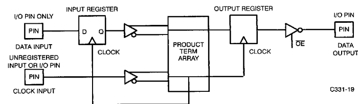
Figure 3. Timing Configurations
