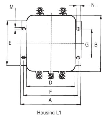
Housing L1
