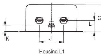
Housing L1
