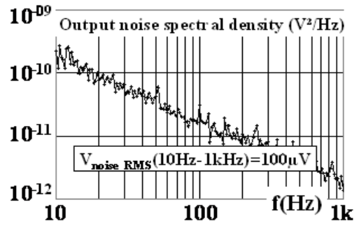
Figure 8: S_{\text{Vout}}(\text{V}^2/\text{Hz}) @ 25^{\circ}\text{C} , I_{\text{Load}}=100\text{mA}
