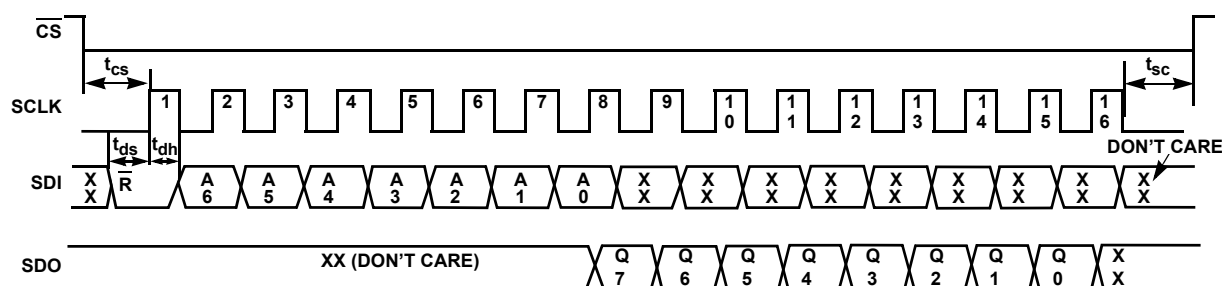
FIGURE 12. READ ON-CHIP REGISTER WAVEFORMS
