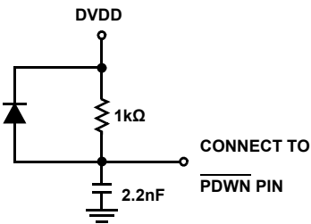
FIGURE 14. PDWN DELAY CIRCUIT
