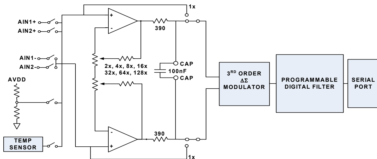
FIGURE 7. ISL26102 (2 CHANNEL) BLOCK DIAGRAM
