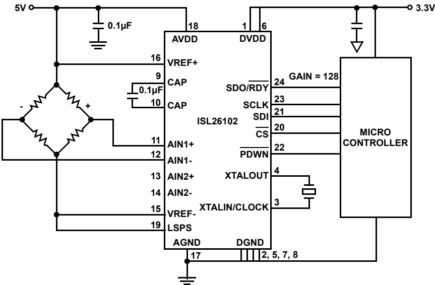
FIGURE 15. A LOAD CELL MEASUREMENT APPLICATION USING THE ISL26102
