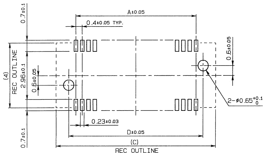
MOUNTING LAYOUT
