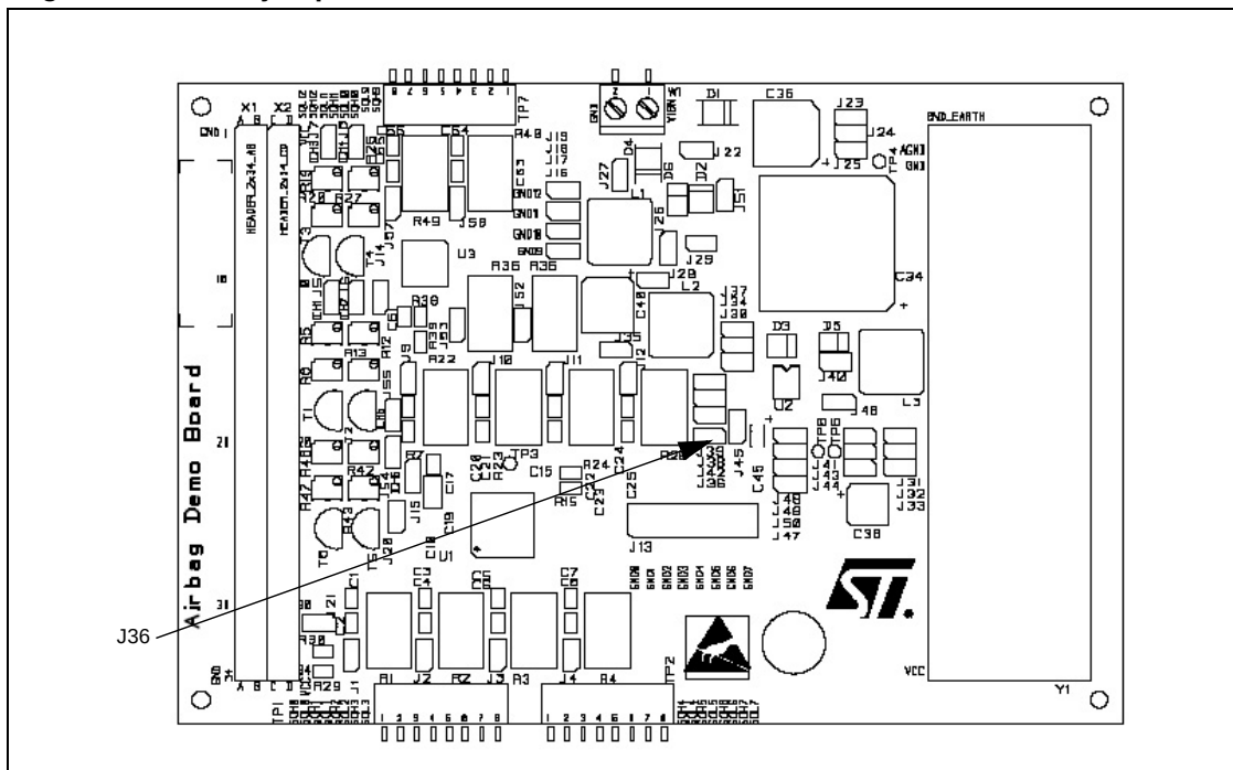
Figure 10. Reset jumper
