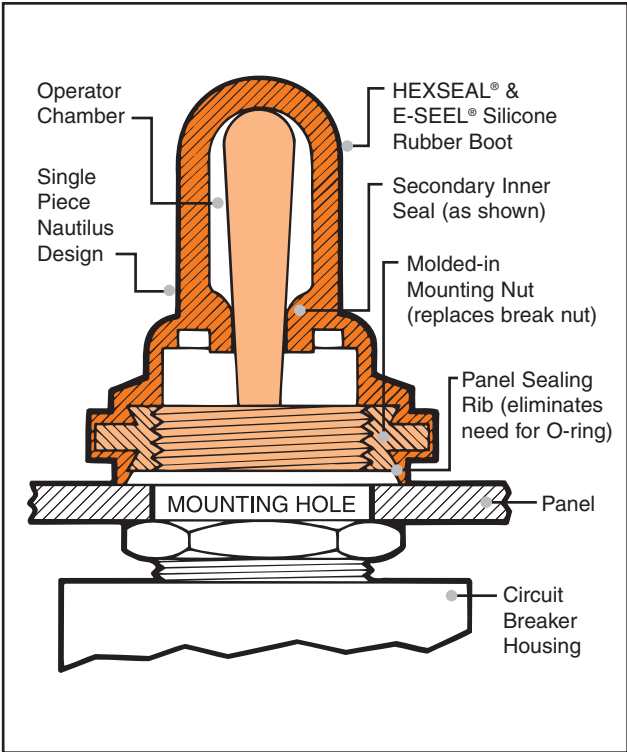
Full-Toggle Boot with Integral Secondary Inner Seal – IP66/68 Rated
