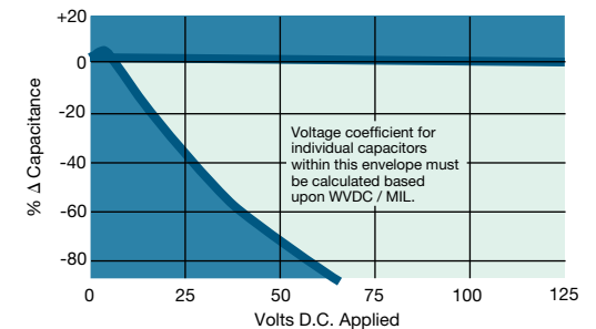
Voltage Coefficient
