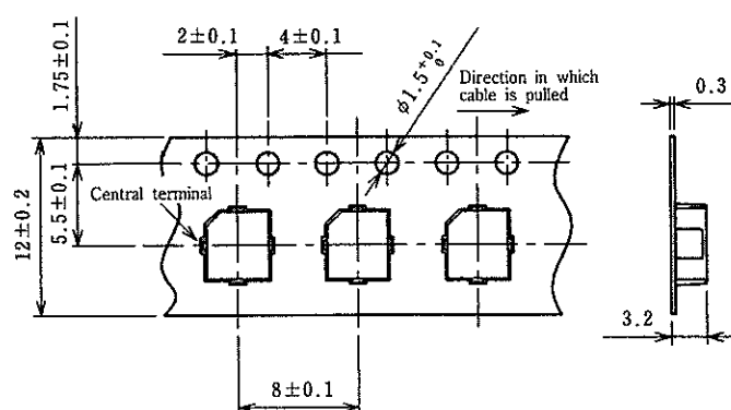
Emboss tapping specifications
