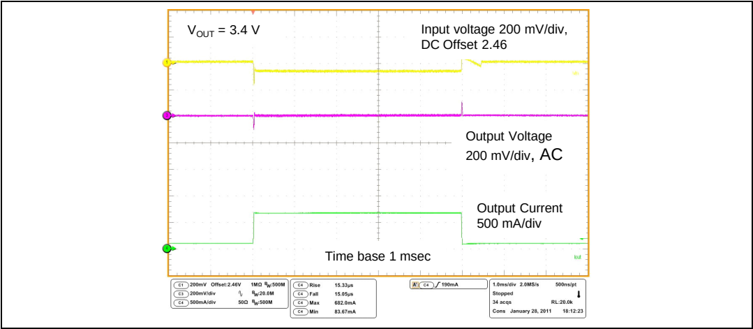
Figure 14. V_{IN} = 2.4\text{ V} , V_{OUT} = 3.4\text{ V} , I_{OUT} = from 80 mA to 630 mA
