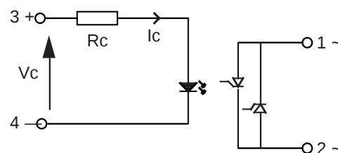
Figure 3 — LS relays
