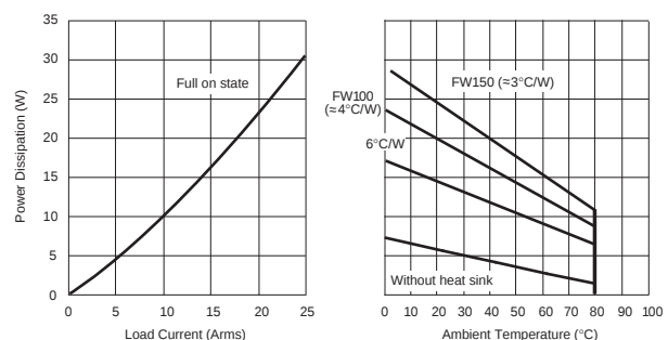
Figure 5b — LS60D22C relays
