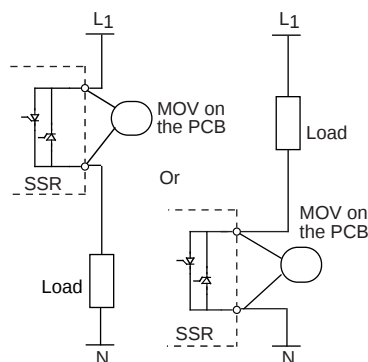
Figure 2 — LS relays
