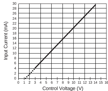
Figure 4 — LS relays
