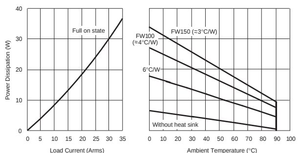
Figure 5c — LS24D27C, LS60D30C relays
