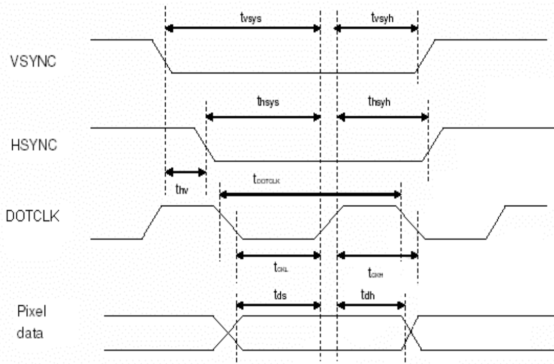
Pixel timing
