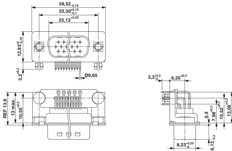
Dimensioned drawing
