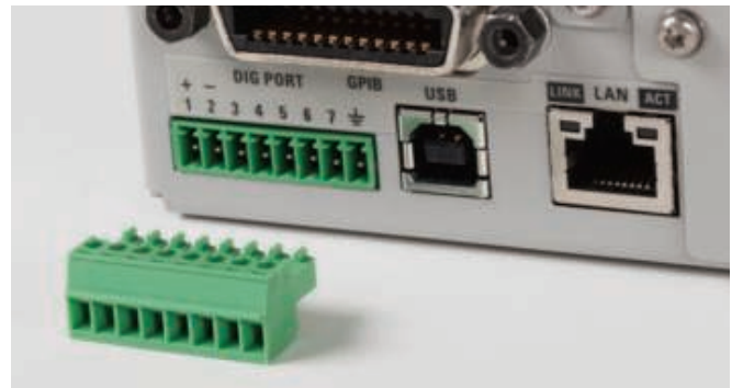
Figure 11. Digital control port on rear panel
