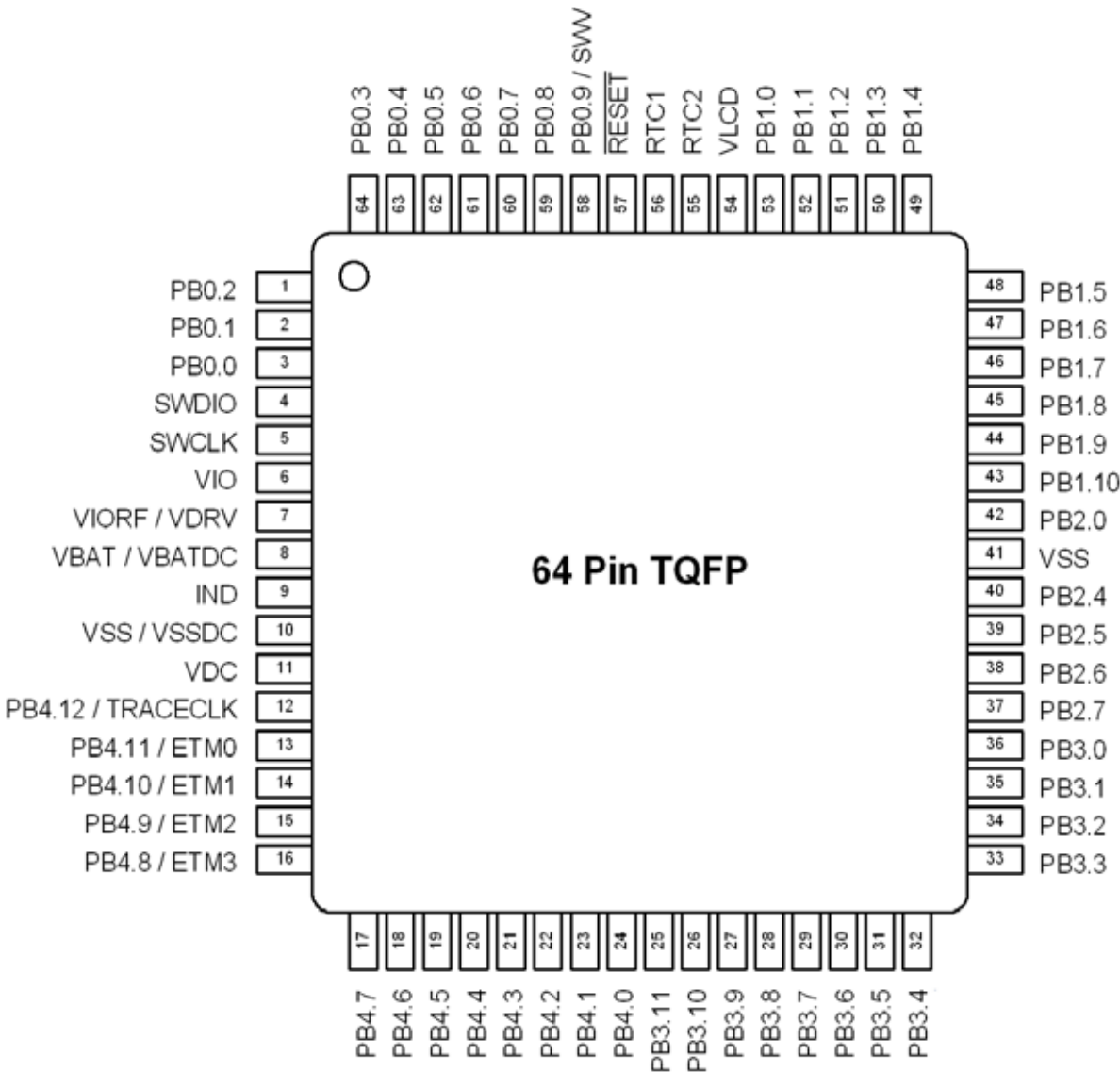
Figure 6.2. SiM3L1x6-QG Pinout
