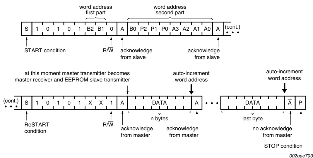
Fig 8. Master reads PCA24S08 slave after setting word address (write word address: read data); sequential read
