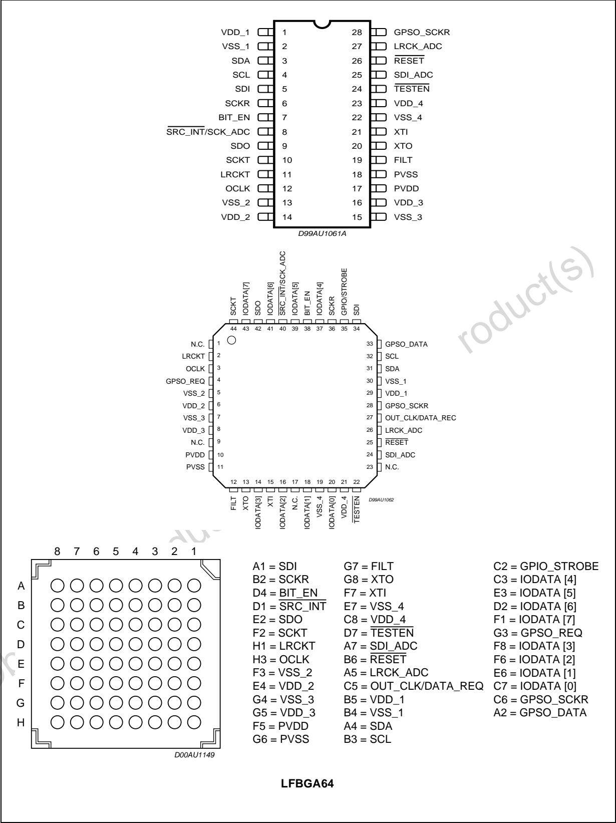
Figure 2. Pin Connection
