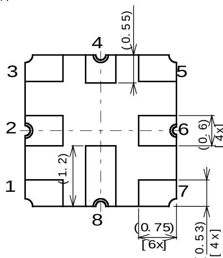
Fig.2 Package dimensions (in mm)
